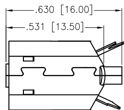
USB-C31-PLUG-B-S1-BK
