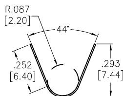
USB-C31-PLUG-B-S2-BK
