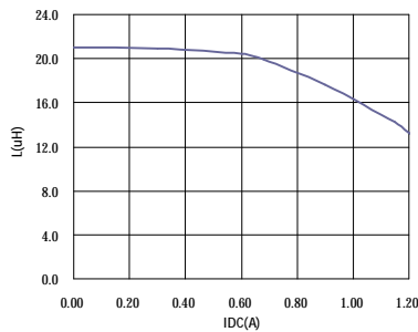
SU5028101Y2□
