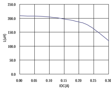
SU5028221Y2□
