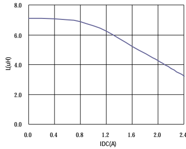
SU5028220Y2□
