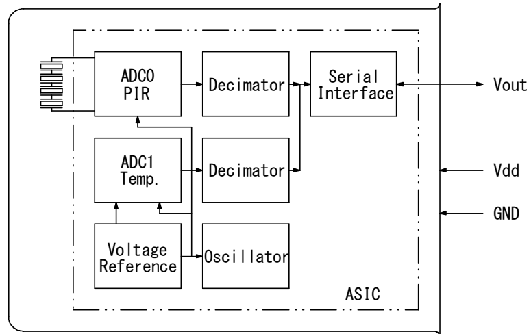
Fig.3 : Circuit Configuration
