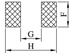
( PCB Pattern )
