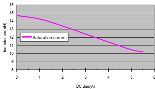
CIP0630LR150M
