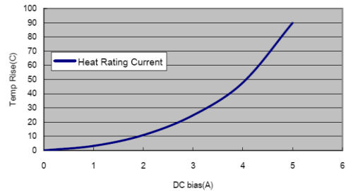
CIP0630LR150M
