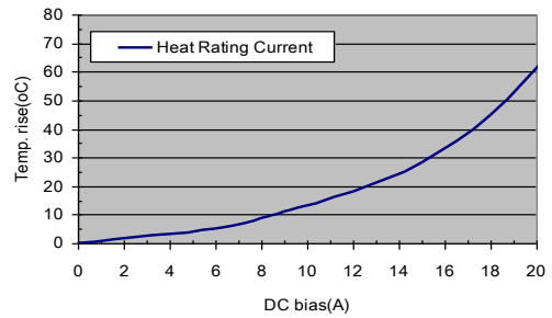
CIP0630LRR68
