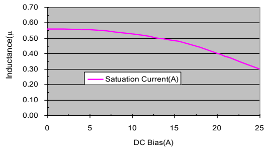
CIP0630LRR56
