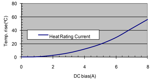
CIP0630LR5R6
