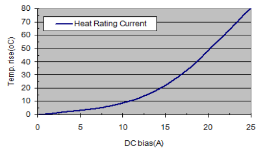
CIP0630LRR47
