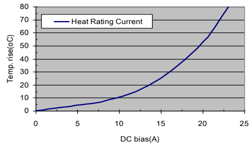
CIP0630LRR56
