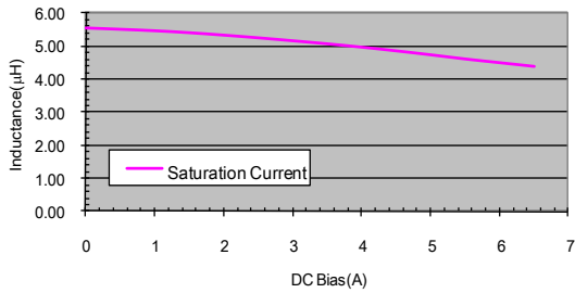
CIP0630LR5R6
