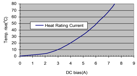
CIP0630LR100
