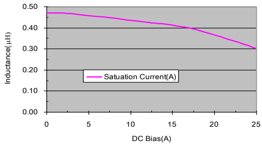
CIP0630LRR47
